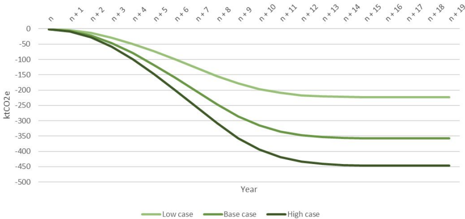
Figure 32: Change in methane emissions nationally in the low, base and high case.
